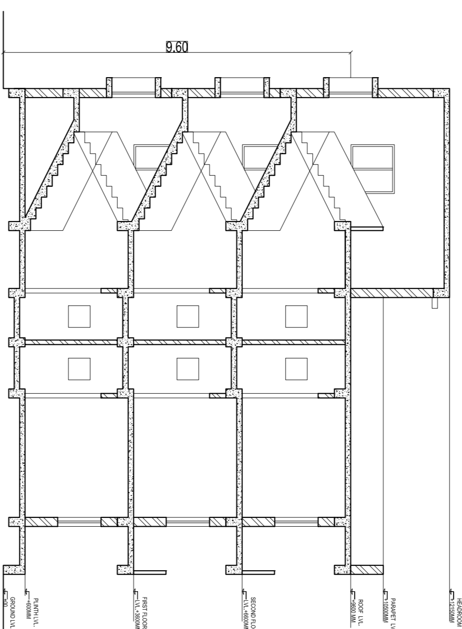
SECTION AA
