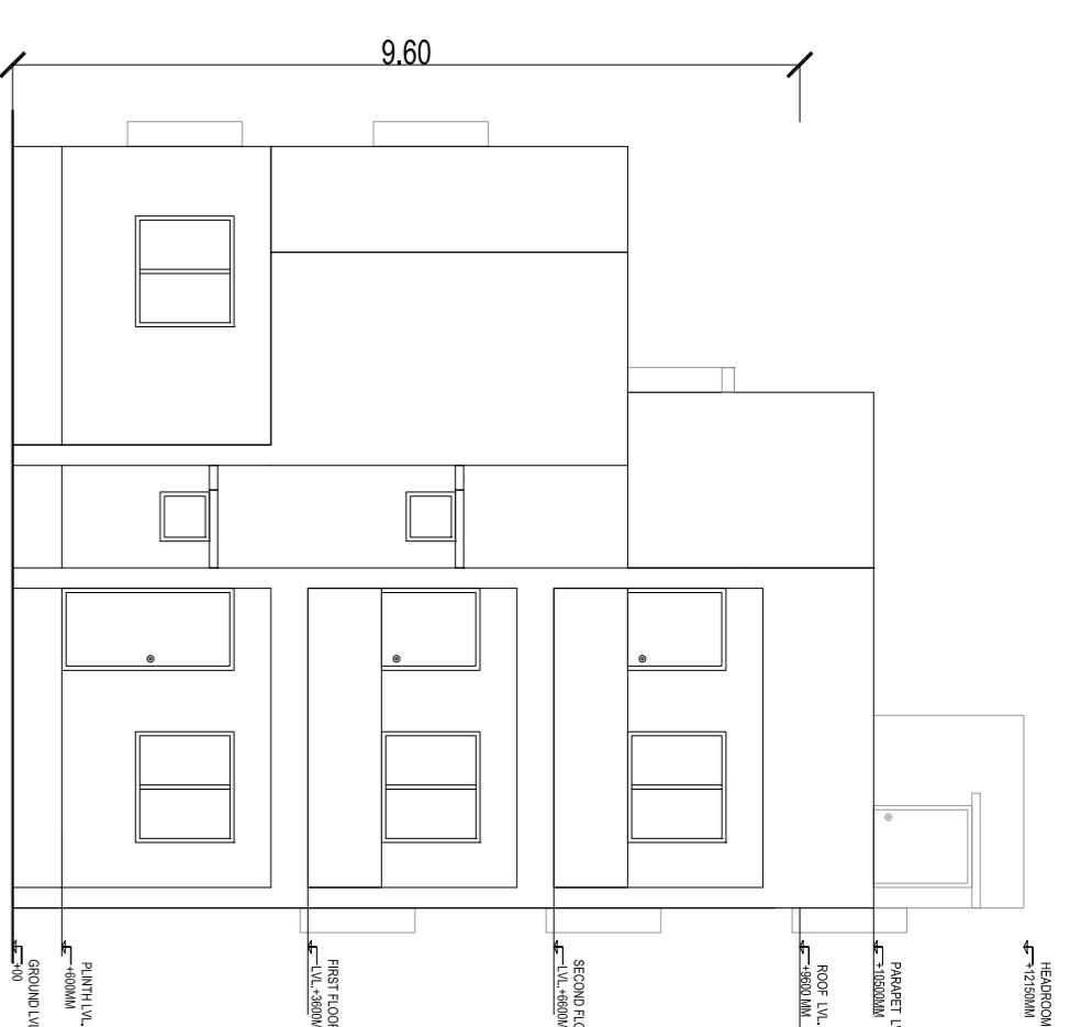
REAR ELEVATION
