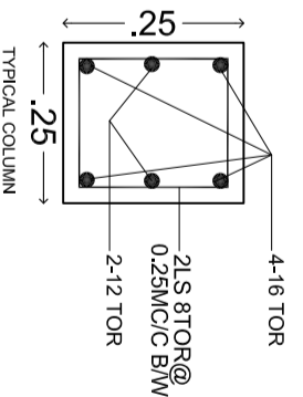
FOUNDATION DETAIL
